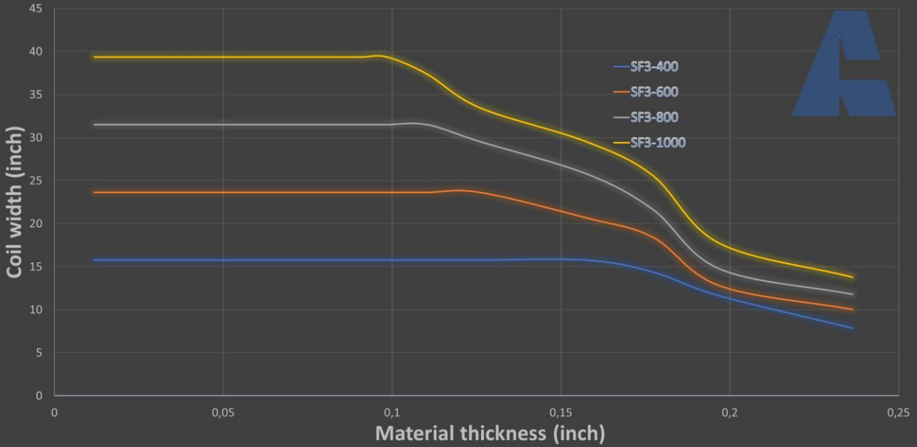
Straightening Capacities for AZ-SF3 models
