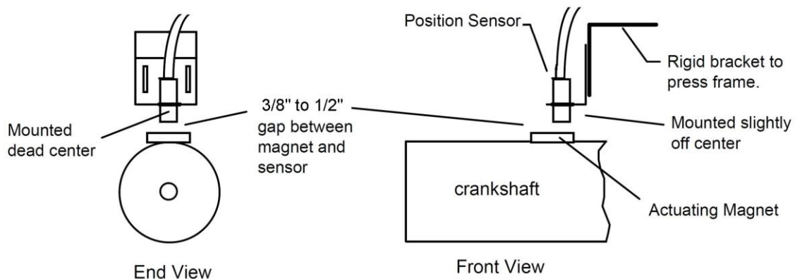
Figure 2-15. How to install the position sensor
