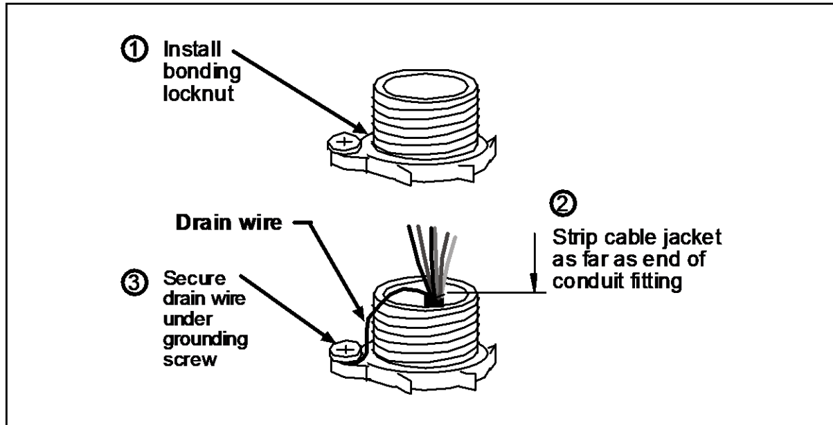
Figure 2-2. Terminating a Cable Shield without Grounding Stud
