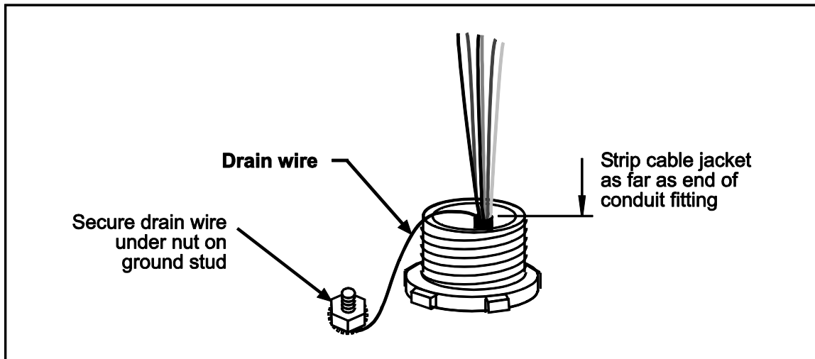
Figure 2-1 Terminating cable shield with and without ground stud
