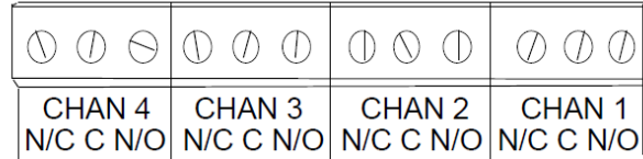
Figure 2-13. Connectors TB302 and TB303 for wiring from relays to equipment
