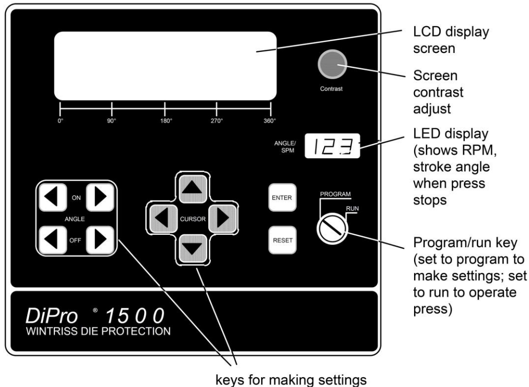
Figure 1-1. DiPro front panel
