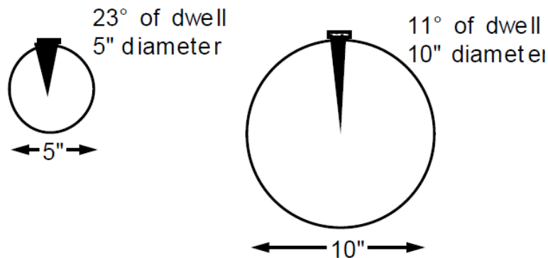
Figure 2-16. Position sensor dwell on different diameter shafts
