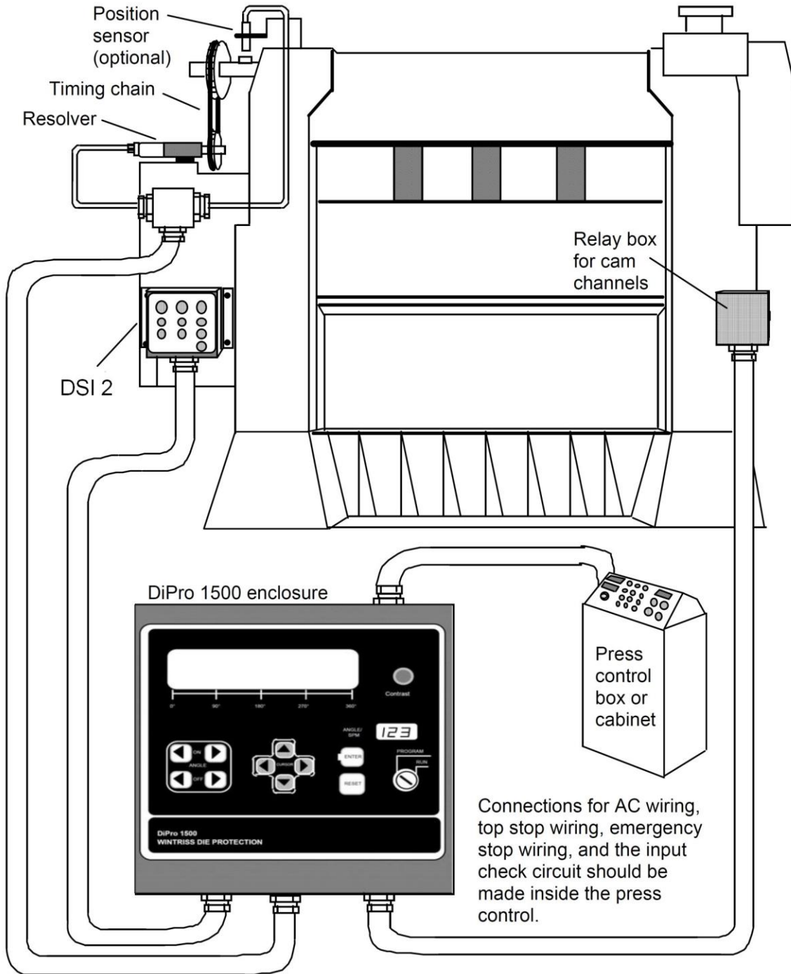
Figure 2-3. Wiring scheme for DiPro 150
